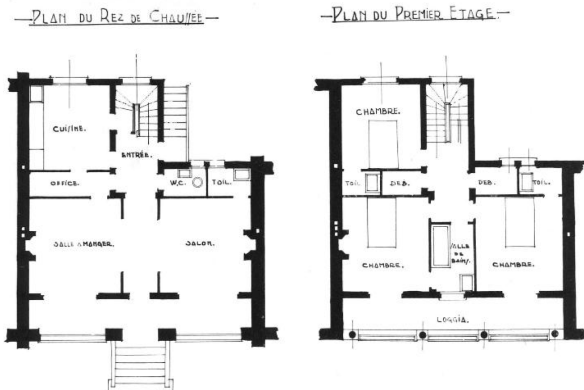
Plans de la villa Plaisance.
