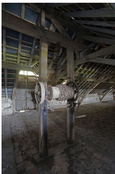
Ecurie-grange, comble : treuil. Phot. Yves Guillotin IVR52_20095300337NUCA
