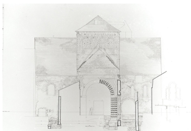
Abbatiale, coupe transversale nef côté transept, 1953. Dessin, in : FORSYTH, George H, The church of St. Martin at Angers, Princeton, University Press, 1953, planche VI. Repro. Patrice Giraud IVR52_19824902452X
