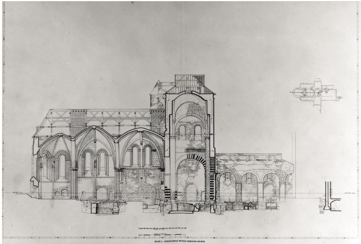
Planche II : coupe longitudinale, 2e quart 20e siècle. Dessin, in : FORSYTH, George H, The church of St. Martin at Angers, Princeton, University Press, 1953, planche VI.
