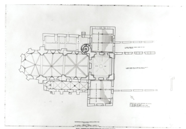
Abbatiale, plan des voûtes, dessin, 1953, in : FORSYTH, George H, The church of St. Martin at Angers, Princeton, University Press, 1953, planche IX. Repro. Patrice Giraud IVR52_19824902420P
