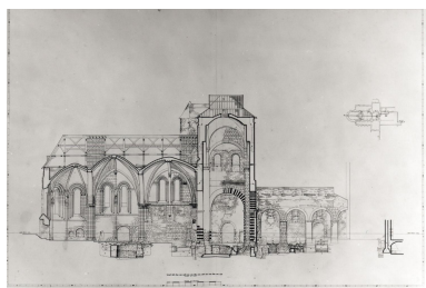
Planche II : coupe longitudinale, 2e quart 20e siècle. Dessin, in : FORSYTH, George H, The church of St. Martin at Angers, Princeton, University Press, 1953, planche VI. Repro. Patrice Giraud IVR52_19824902418P
