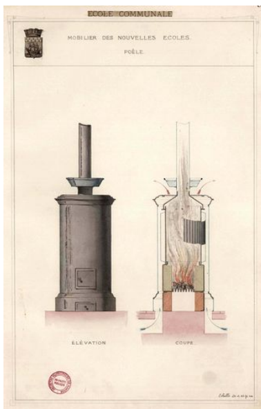
Plan du poêle, 1878. Phot. Patrick (reproduction) Jean IVR52_20124400452NUCA
